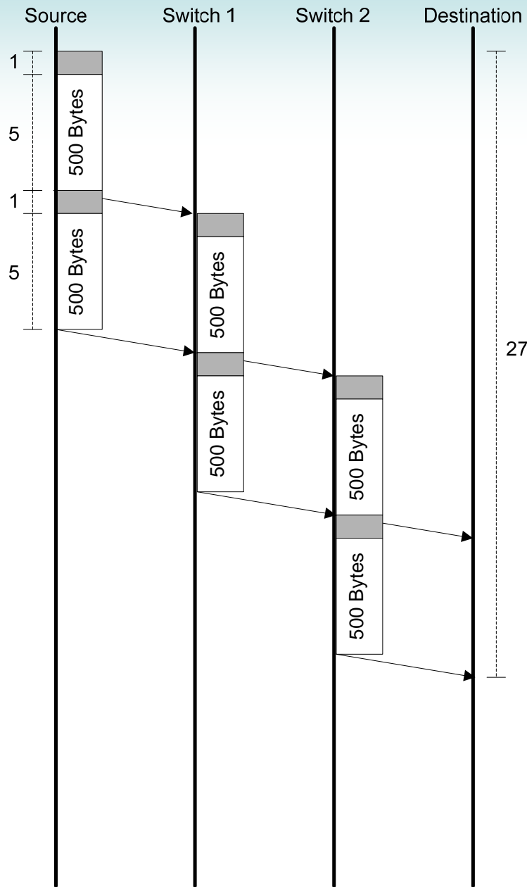
2 packets per message, 3 links
