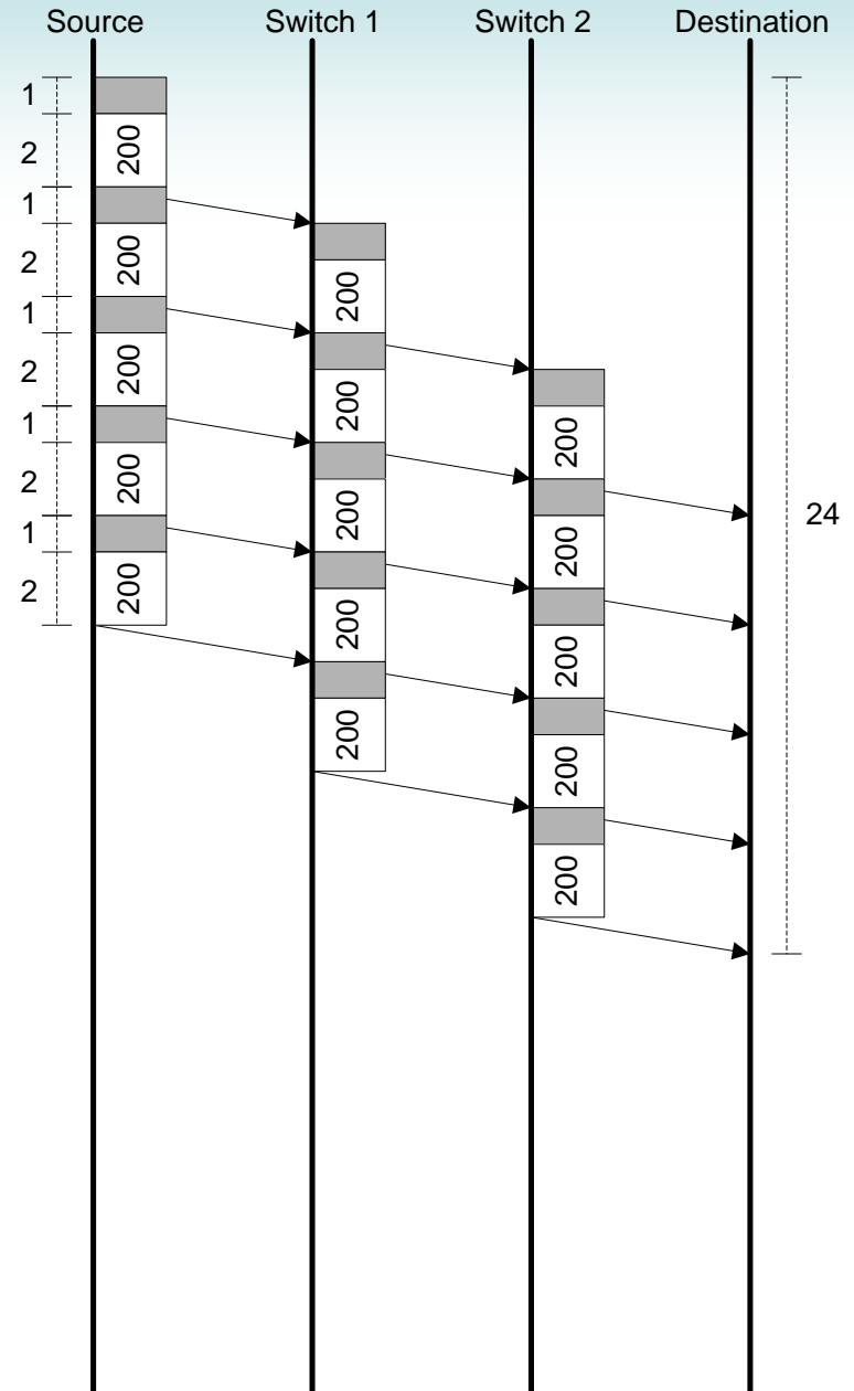
5 packets per message, 3 links
